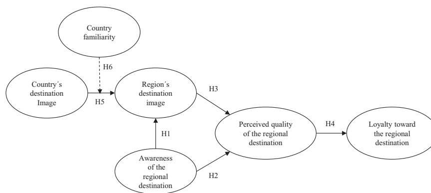
Fig. 1. Theoretical model.
