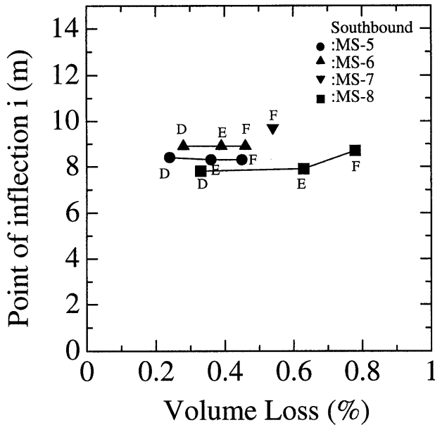
Fig. 18. Relationship between volume loss and i
