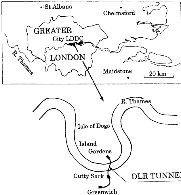
Fig. 1. Route of DLR-LWE TUNNEL
