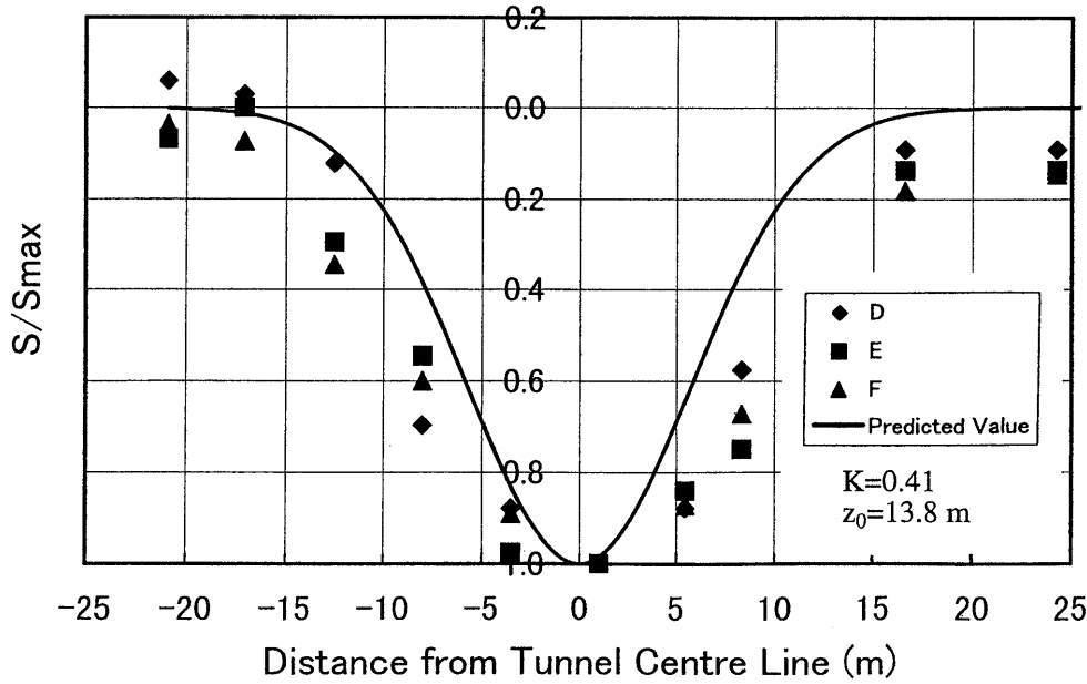
Fig. 9(a). Transverse settlement troughs ( S/S_{max} vs. y )
