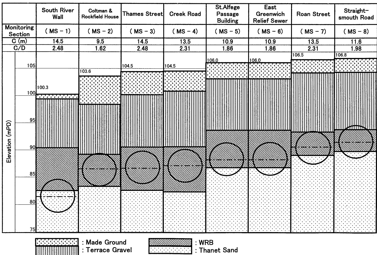
Fig. 3. Ground conditions at monitoring sections
